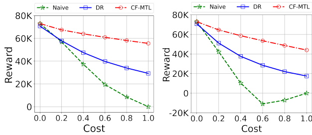
(a) Reward on YELP with coupon incentives.
